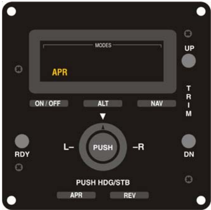
Fig. 2-20. AP Display, APR Mode Engaged (System Fifty)
